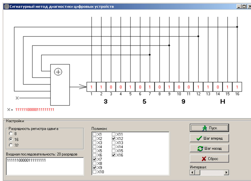
Figure 2. Digital signature after the end of the process.
